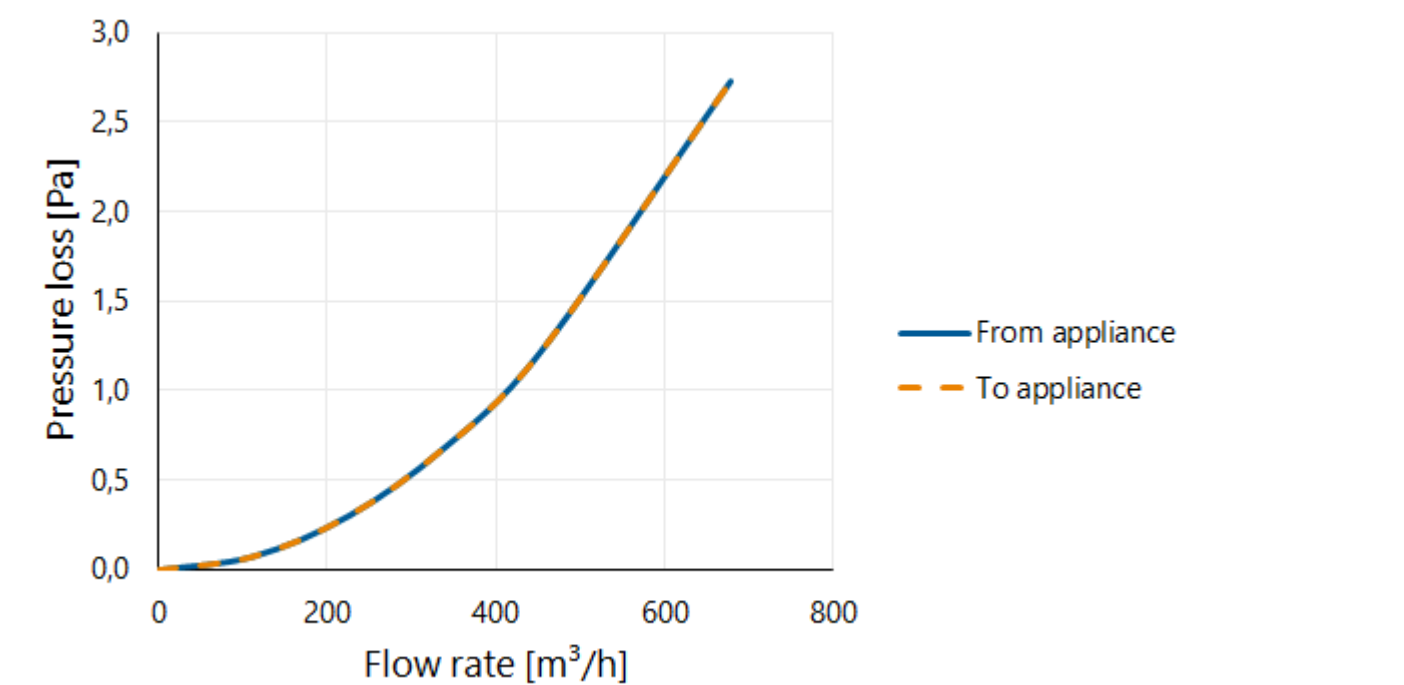
Pressure loss
