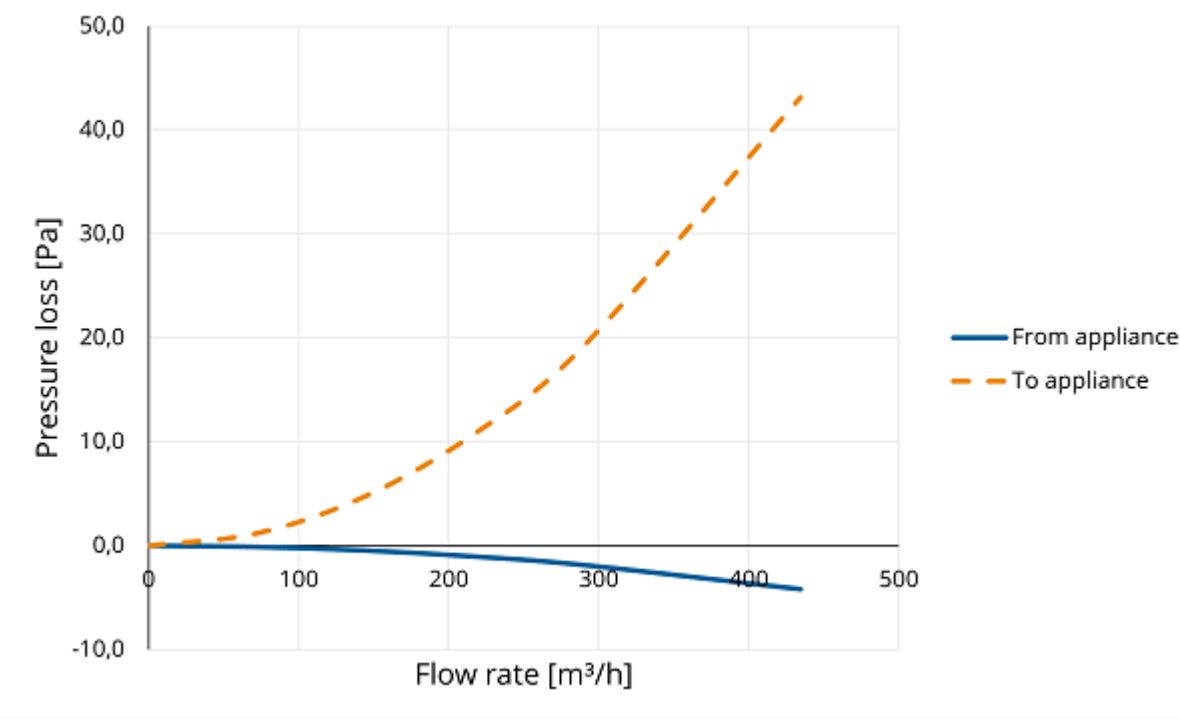
Pressure loss
