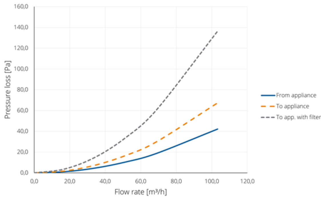
Pressure loss
