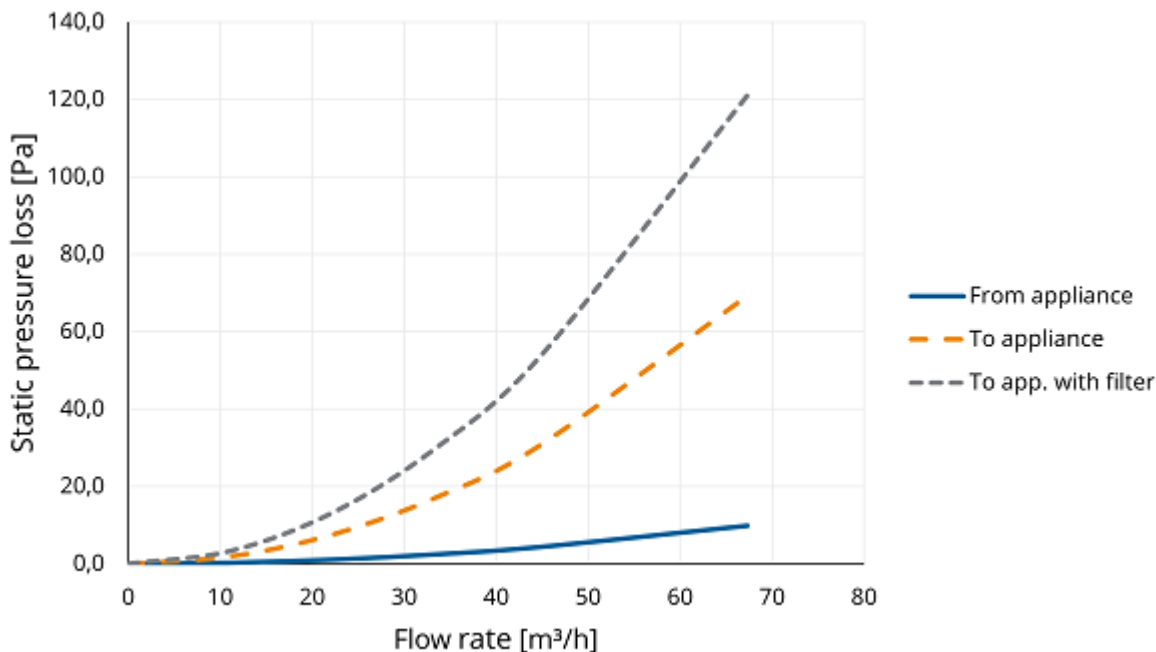
Pressure loss
